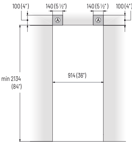
A Area to be left clear for the anti-tipping brackets
