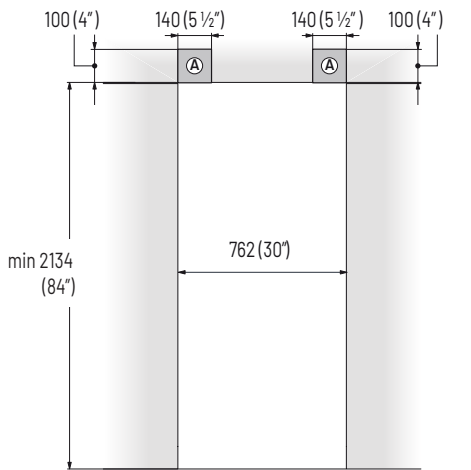
A Area to be left clear for the anti-tipping brackets
